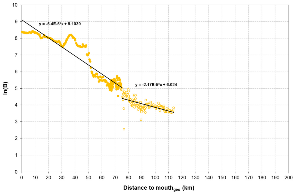
Figure A 4 – Convergence for the Humber-Ouse estuary. 1/b values are given in Table 4
