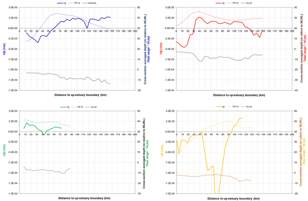
Figure 24 – Tidal damping ( 1/\beta ) (averaged over 5 km blocks) for the Scheldt (blue), Elbe (red), Weser (green) and Humber-Ouse (yellow)
