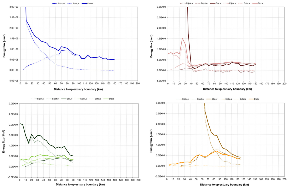
Figure 25 – Energy fluxes (tidal = E_{tj,tot} , fluvial = E_{q,tot} and total = E_{tot} , averaged over 5 km blocks) along the Scheldt (blue), Elbe (red), Weser (green) and Humber-Ouse (yellow), under high (winter) and low (summer) freshwater discharge conditions. For the Scheldt, energy fluxes are only calculated under mean freshwater discharge conditions
