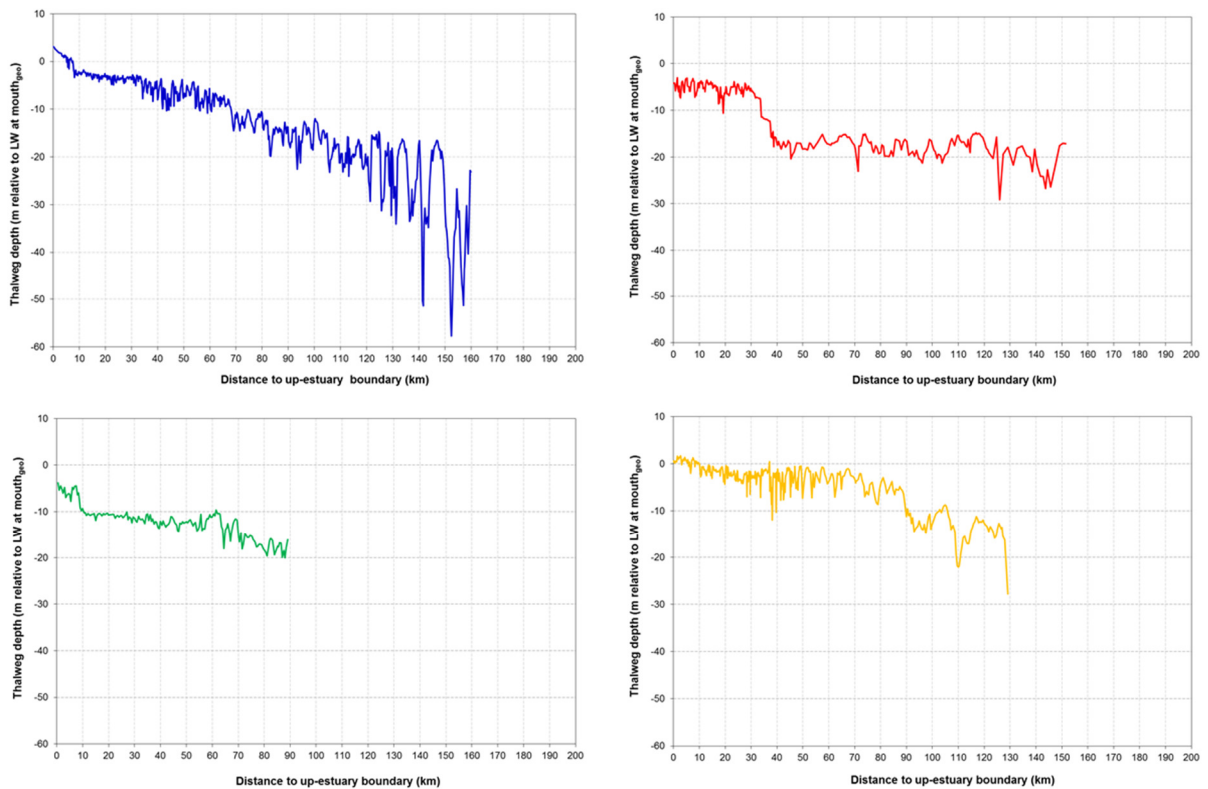
Figure 14 – Thalweg depth for the Scheldt (blue), Elbe (red), Weser (green) and Humber-Ouse (yellow), relative to low water level at mouth geo
