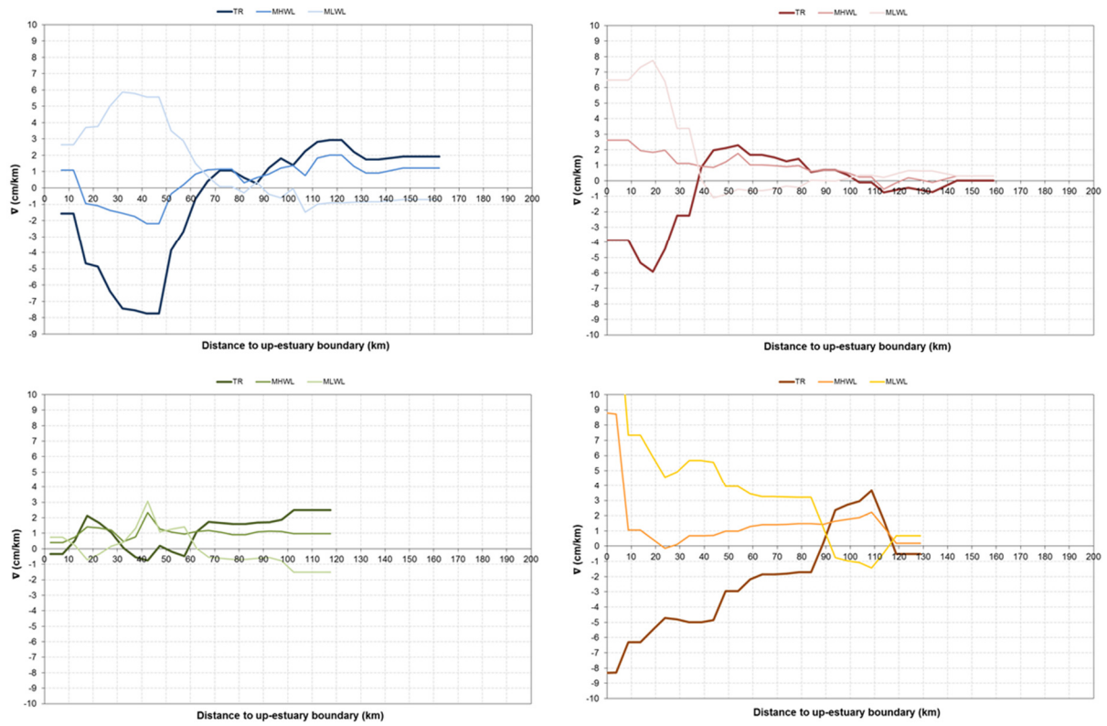
Figure 19 – Gradient (averaged over 5 km blocks) for the tidal range, MHWL and MLWL, for the Scheldt (blue), Elbe (red), Weser (green) and Humber-Ouse (yellow)
