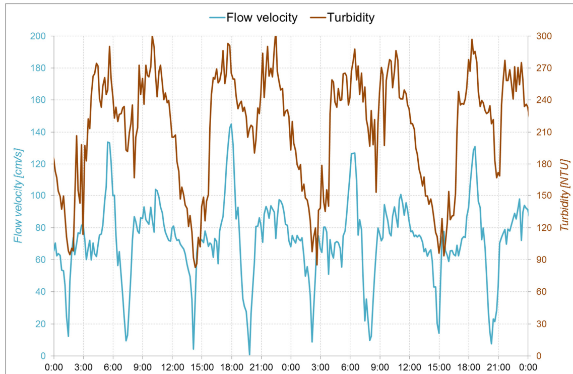
Figure 6 – Variation of flow velocity and SPM (turbidity) over tidal cycle for station Oosterweel (Scheldt estuary)
